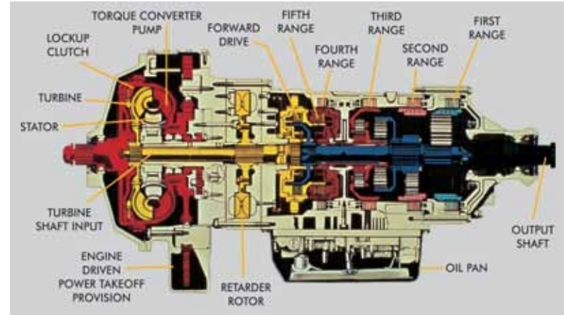
CL(B)T 754 Transmission Cut section
