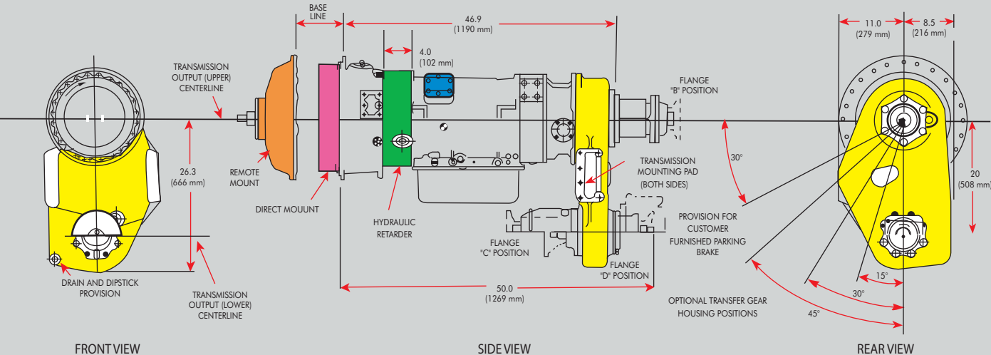
Mounting Dimensions - Drop Box Model
